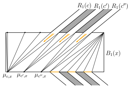
Figure 7: A triangulation for B_1(x) , where x = \text{true} .
